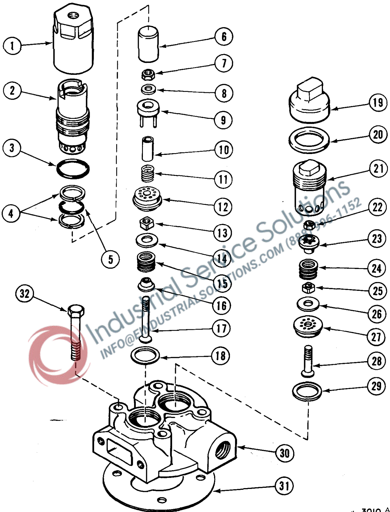
Group No. 2 CYLINDER HEAD, High Pressure
